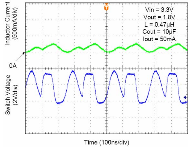
Discontinuous Current
