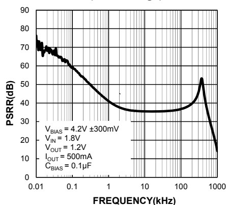
Power Supply Rejection Ratio (Bias Voltage)
