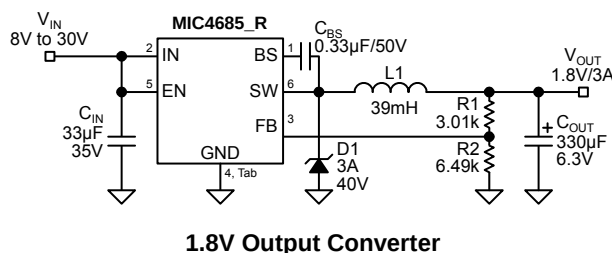
1.8V Output Converter
