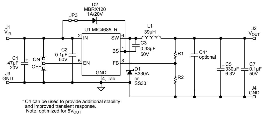
Figure 3. Schematic Diagram
