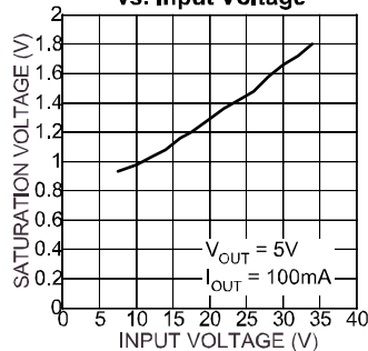
Saturation Voltage vs. Input Voltage
