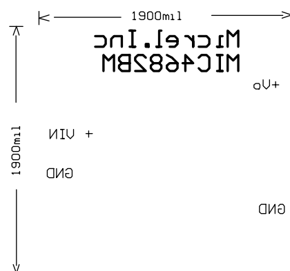
Figure 5d. Bottom Silkscreen
