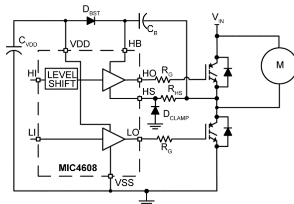
Figure 6. MIC4608 Driving a Motor
