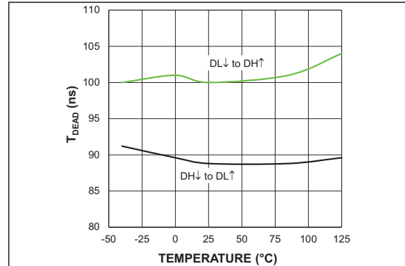
FIGURE 3-16: Deadtime Delay vs. Temperature.
