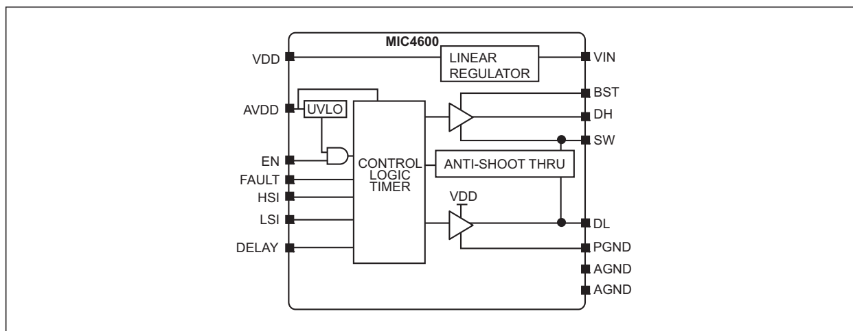
FIGURE 4-1: Functional Diagram.
