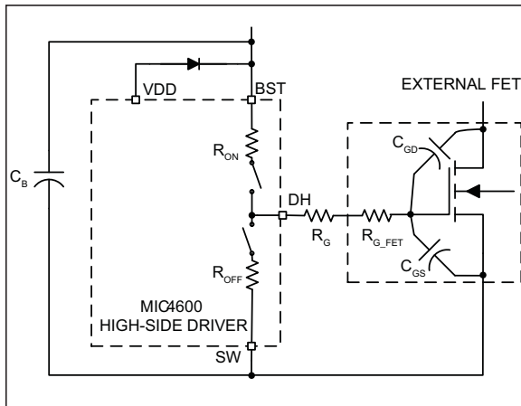
FIGURE 6-1: MIC4600 Driving an External MOSFET.
