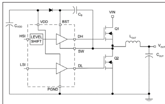
FIGURE 4-4: MIC4600 Driving a Synchronous Buck Converter.
