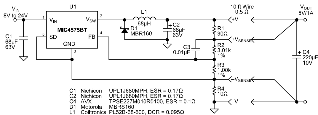
Figure 19. Remote-Sensing Regulator
