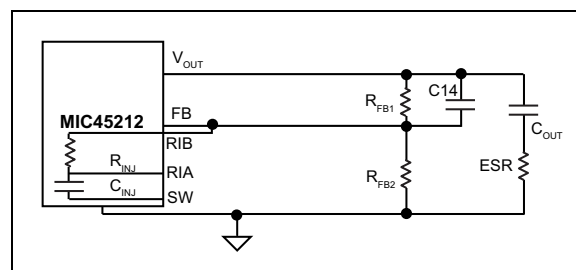
FIGURE 5-5: Internal Ripple Injection at FB via RIB Pin.
