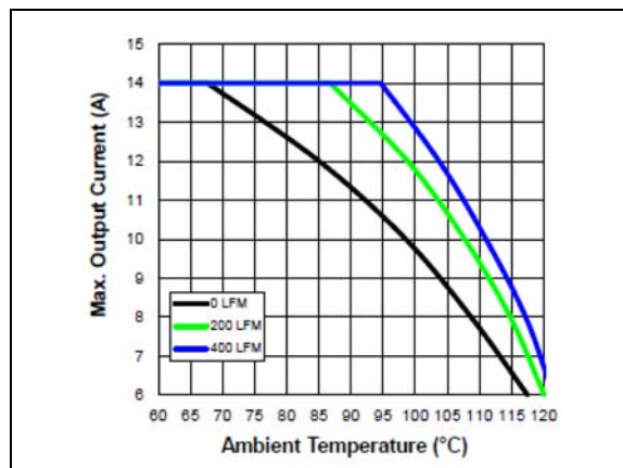
FIGURE 5-6: MIC45212 Power Derating vs. Airflow (60 V IN to 1.5 V OUT ).
