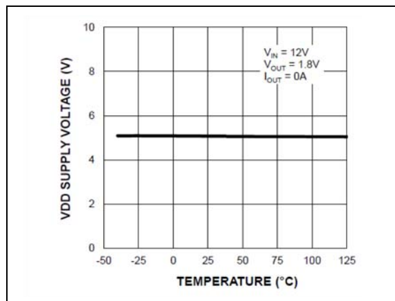
FIGURE 2-4: V_{DD} Supply Voltage vs. Temperature.
