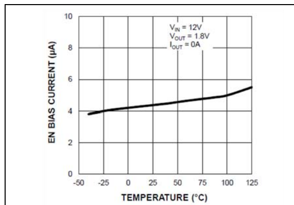
FIGURE 2-6: EN Bias Current vs. Temperature.
