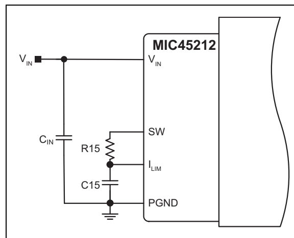
FIGURE 4-5: MIC45212 Current-Limiting Circuit.
