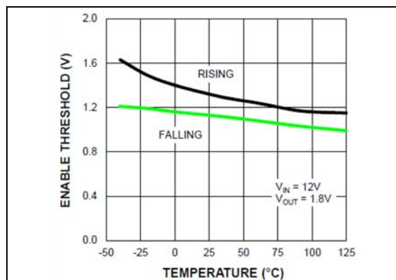
FIGURE 2-5: Enable Threshold vs. Temperature.
