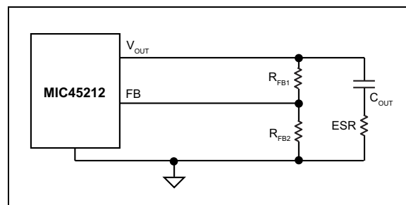
FIGURE 5-4: Enough Ripple at FB from ESR.
