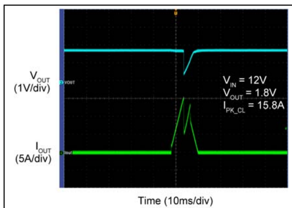
FIGURE 2-32: Peak Current-Limit Threshold.
