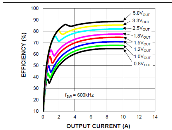
FIGURE 2-16: Efficiency ( V_{IN} = 24V ) vs. Output Current (MIC45208-2).
