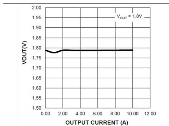
FIGURE 2-17: Load Regulation vs. Input Voltage.
