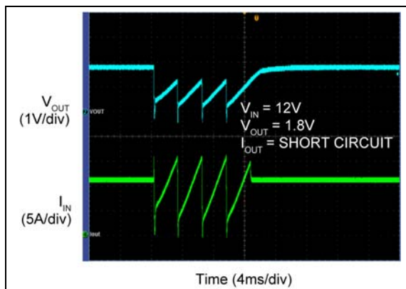
FIGURE 2-31: Output Recovery from Short Circuit.
