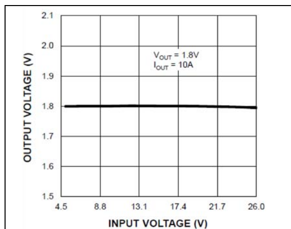
FIGURE 2-18: Line Regulation.
