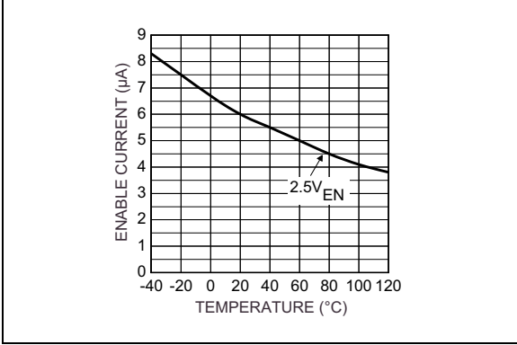
FIGURE 2-29: Enable Current vs. Temperature.
