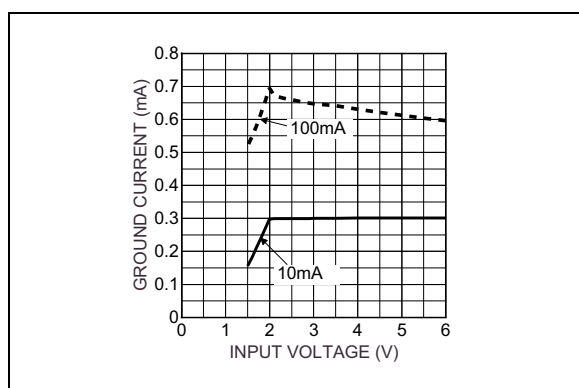
FIGURE 2-14: Ground Current vs. Supply Voltage (1.8V).
