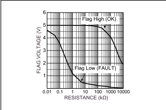
FIGURE 2-28: Error Flag Pull-Up Resistor.
