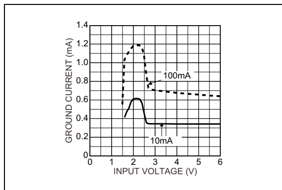
FIGURE 2-16: Ground Current vs. Supply Voltage (2.5V).
