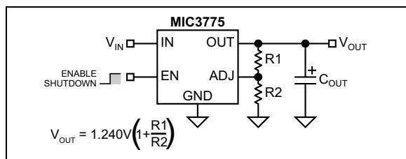
FIGURE 4-2: Adjustable Regulator with Resistors.
