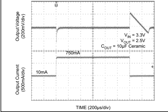
FIGURE 2-30: Load Transient Response.
