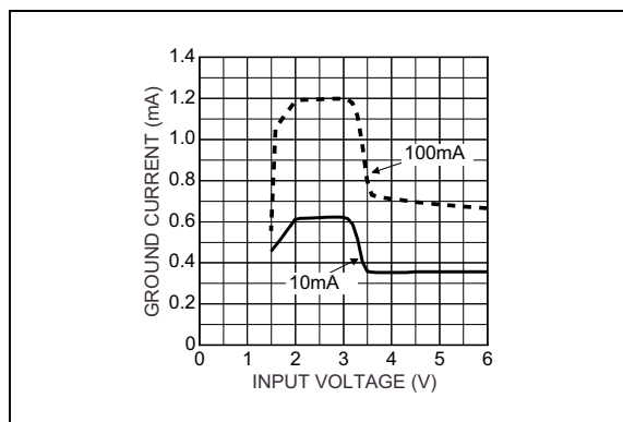
FIGURE 2-18: Ground Current vs. Supply Voltage (3.3V).
