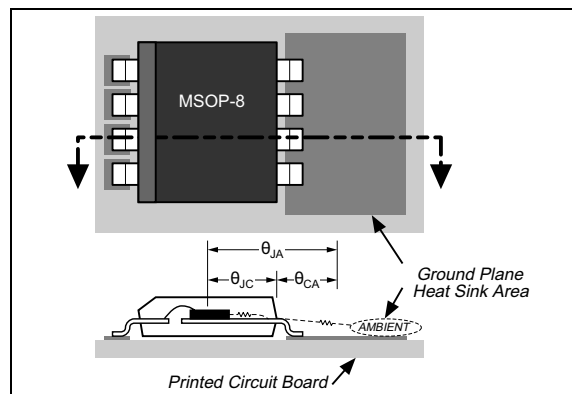
FIGURE 4-3: Thermal Resistance.
