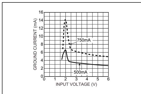
FIGURE 2-15: Ground Current vs. Supply Voltage (1.8V).
