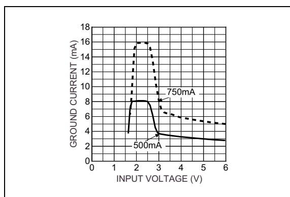
FIGURE 2-17: Ground Current vs. Supply Voltage (2.5V).
