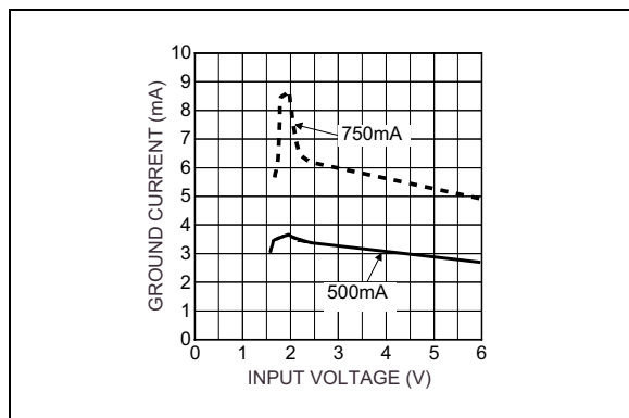
FIGURE 2-13: Ground Current vs. Supply Voltage (1.5V).
