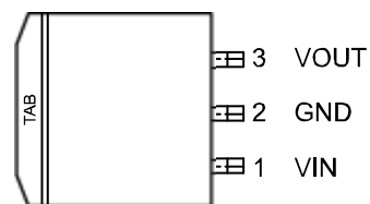
S-PAK-3 (R)
