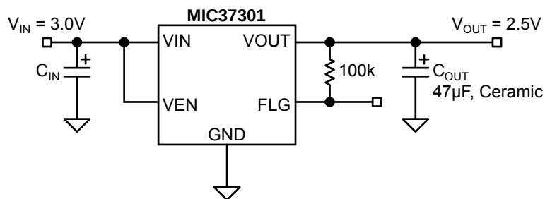
Fixed 2.5V Regulator with Error Flag
