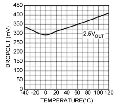
FIGURE 2-4: Dropout vs. Temperature.
