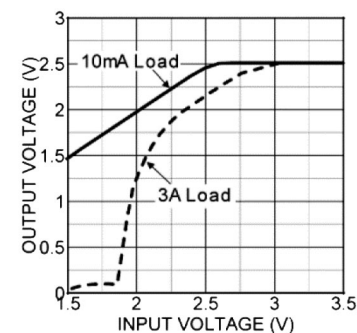
FIGURE 2-6: Dropout Characteristics (2.5V).
