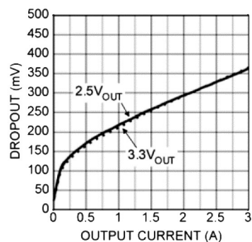
FIGURE 2-3: Dropout vs. Output Current.
