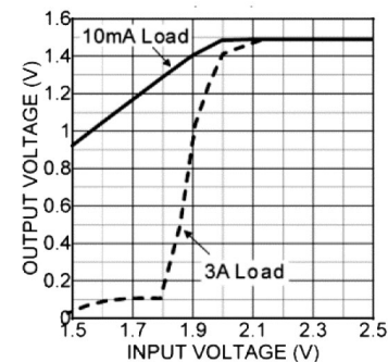
FIGURE 2-5: Dropout Characteristics (1.5V).
