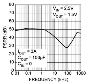
FIGURE 2-2: Power Supply Rejection Ratio.
