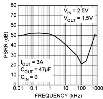
FIGURE 2-1: Power Supply Rejection Ratio.
