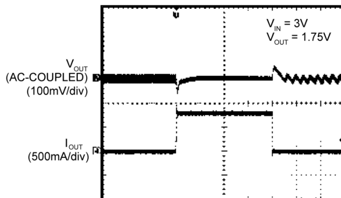
Load Transient (10mA – 750mA)
