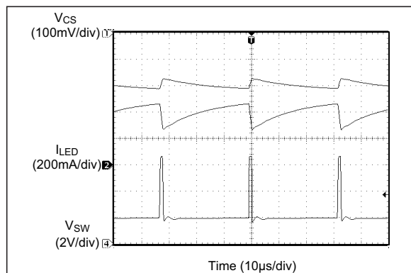
FIGURE 2-25: Steady-State Operation at V_{IN} = 6V .
