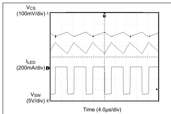
FIGURE 2-27: Steady-State Operation at V_{IN} = 12V .
