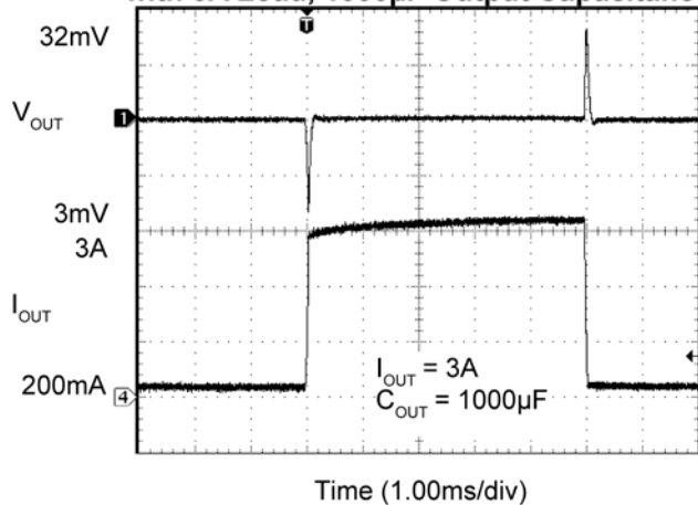
MIC29302A Load Transient Response with 3A Load, 1000μF Output Capacitance
