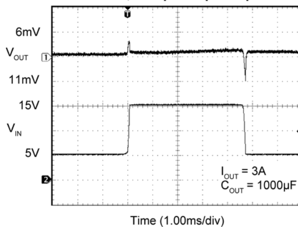
MIC29302A Line Transient Response with 3A Load, 1000μF Output Capacitance
