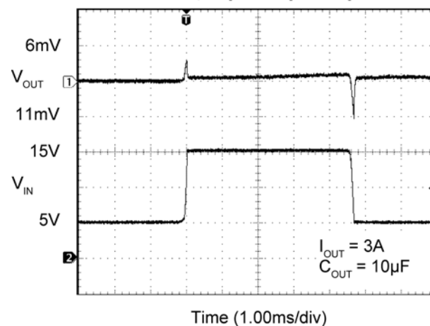
MIC29302A Line Transient Response with 3A Load, 10μF Output Capacitance
