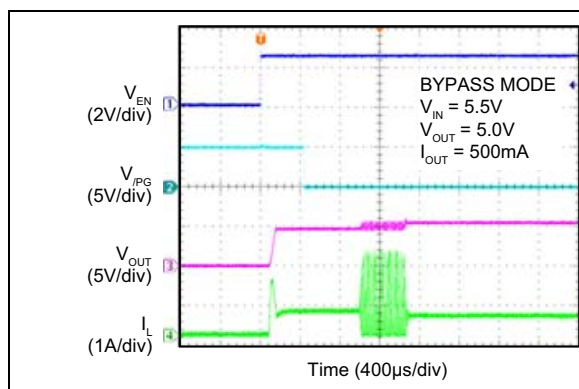
FIGURE 2-19: Soft-Start (Bypass Mode).
