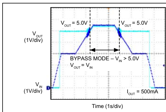
FIGURE 2-21: Bypass Mode.
