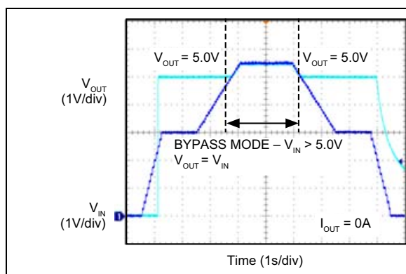
FIGURE 2-20: Bypass Mode.
