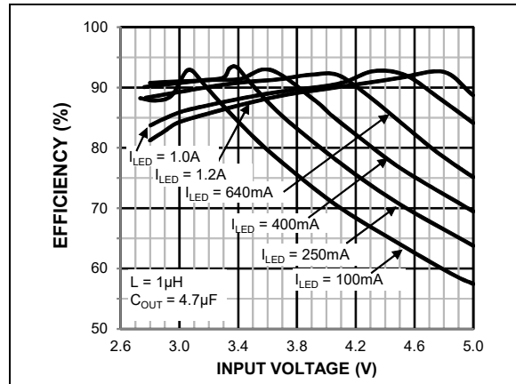
FIGURE 2-4: WLED Power Efficiency vs. Input Voltage.
