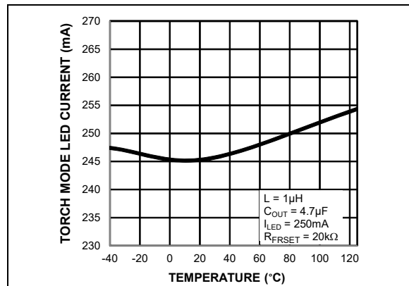
FIGURE 2-5: Torch Mode LED Current vs. Temperature.
