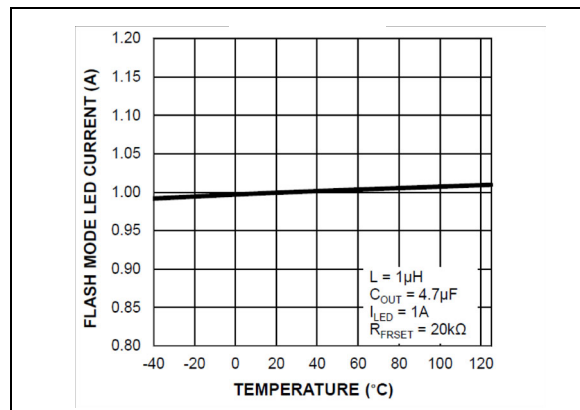
FIGURE 2-6: Flash Mode LED Current vs. Temperature.
