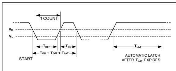
FIGURE 5-2: Data Word Pulse Timing.
