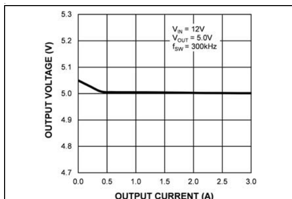
FIGURE 2-10: Output Voltage vs. Output Current (MIC28511-1).
