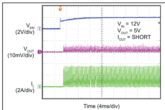
FIGURE 2-45: Enabled into Short.
