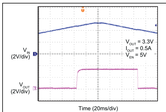
FIGURE 2-43: V_{IN} UVLO Thresholds.
