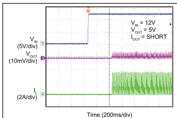
FIGURE 2-44: Power-Up into Short-Circuit.
