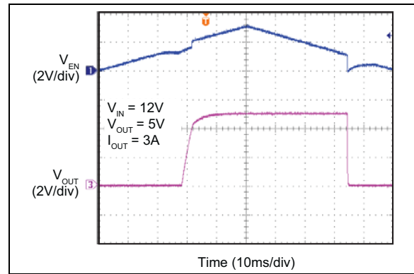
FIGURE 2-42: Enable Turn-On/Turn-Off.
