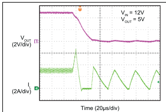
FIGURE 2-47: Short-Circuit.
