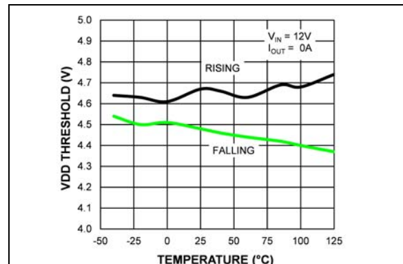
FIGURE 2-6: V_{DD} UVLO Threshold vs. Temperature (MIC28511-1).
