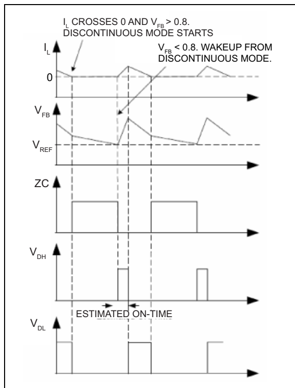
FIGURE 4-4: MIC28511-1 Control Loop Timing (Discontinuous Mode).
