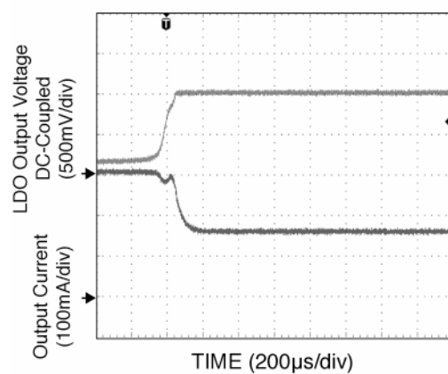
LDO Short Circuit Recovery to 150mA Load
