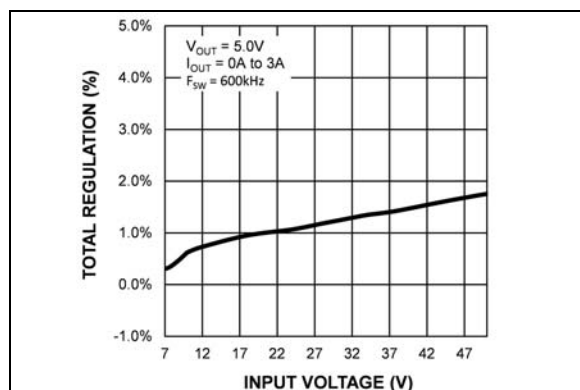
FIGURE 2-5: Output Regulation vs. Input Voltage (MIC28303-1).
