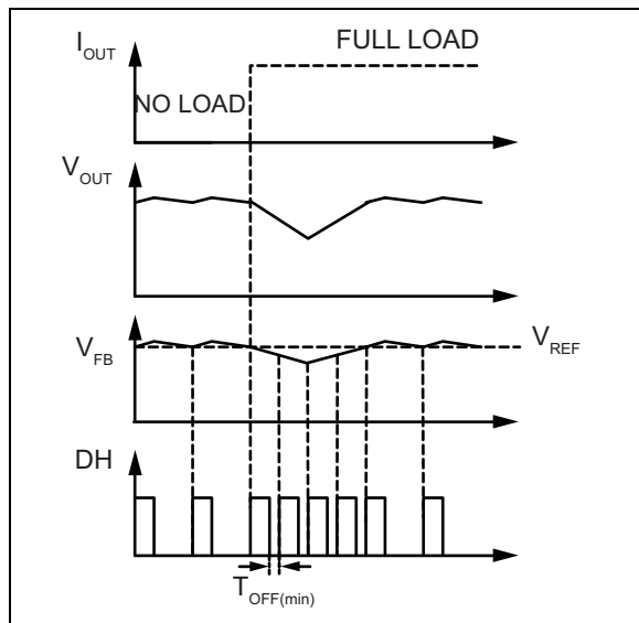
FIGURE 4-2: MIC28303 Load Transient Response
