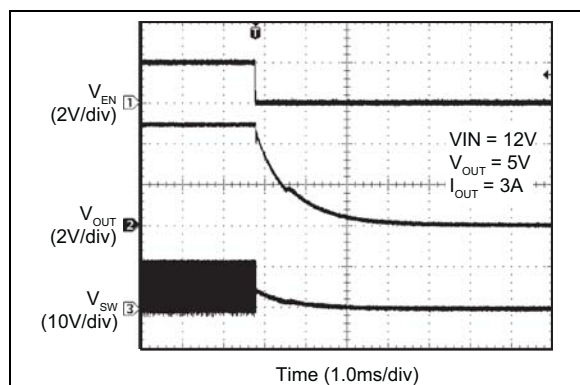
FIGURE 2-40: Enable Turn-Off Delay and Fall Time.
