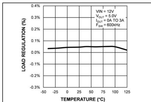
FIGURE 2-26: Load Regulation vs. Temperature (MIC28303-2).
