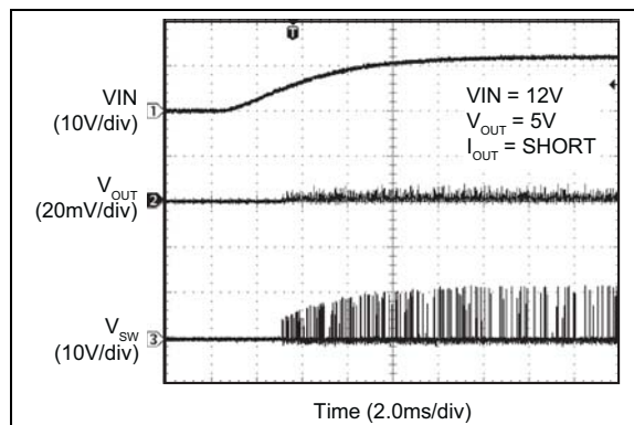
FIGURE 2-46: Power-Up into Short-Circuit.
