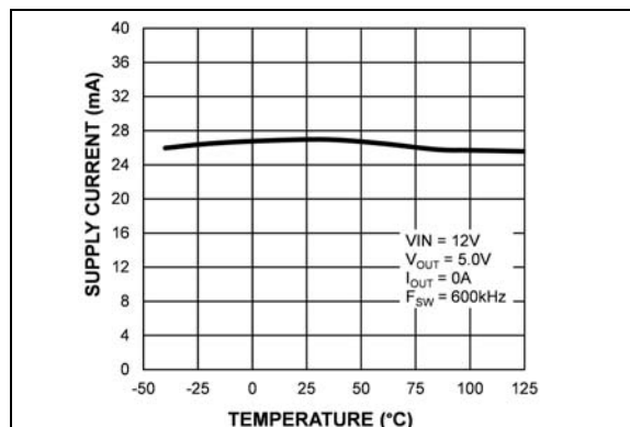
FIGURE 2-25: V_{IN} Operating Supply Current vs. Temperature (MIC28303-2).
