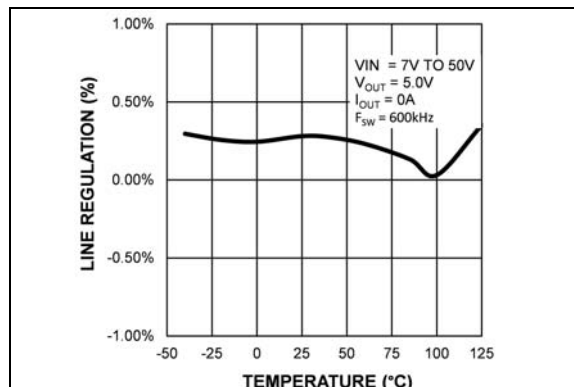
FIGURE 2-27: Line Regulation vs. Temperature (MIC28303-2).
