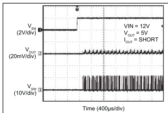
FIGURE 2-47: Enabled into Short.
