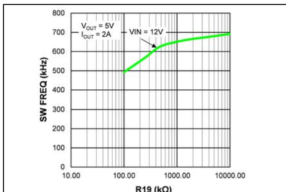
FIGURE 2-34: Switching Frequency.
