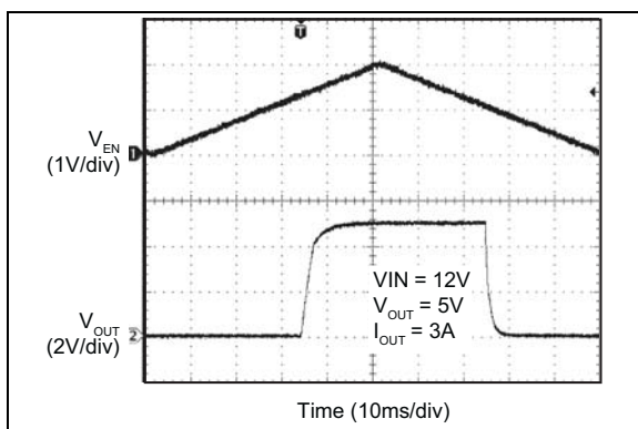
FIGURE 2-44: Enable Thresholds.
