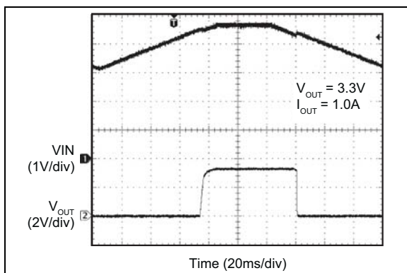
FIGURE 2-45: UVLO Thresholds.
