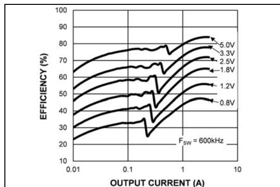
FIGURE 2-13: Efficiency ( V_{IN} = 24V ) vs. Output Current (MIC28303-1).
