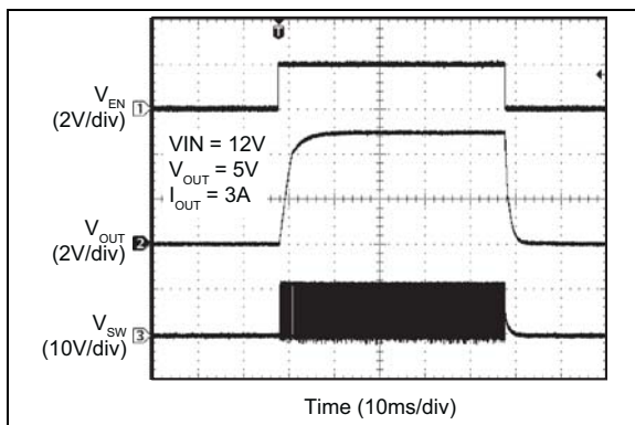
FIGURE 2-43: Enable Turn-On/Turn-Off.
