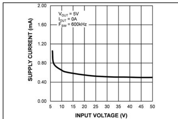
FIGURE 2-4: V_{IN} Operating Supply vs. Input Voltage (MIC28303-1).
