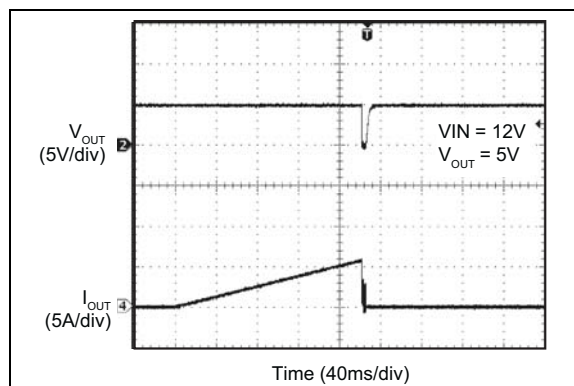
FIGURE 2-48: Output Peak Current-Limit Threshold.
