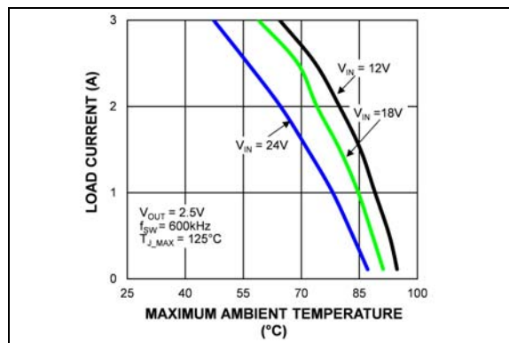
FIGURE 2-37: Thermal Derating (MIC28303-2).
