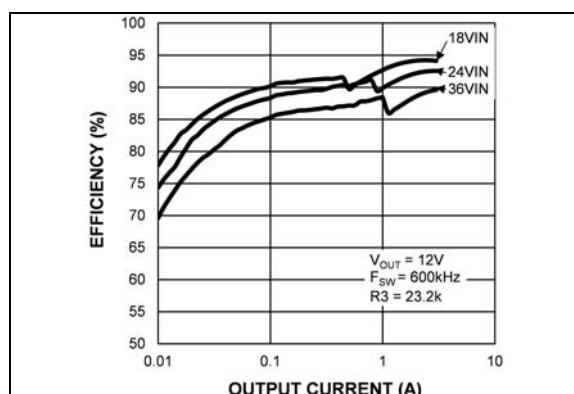
FIGURE 2-14: Efficiency vs. Output Current (MIC28303-1).
