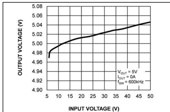
FIGURE 2-6: Output Voltage vs. Input Voltage (MIC28303-1).
