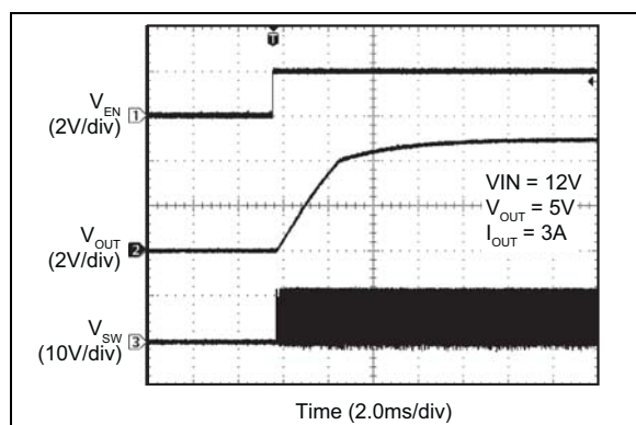
FIGURE 2-39: Enable Turn-On Delay and Rise Time.
