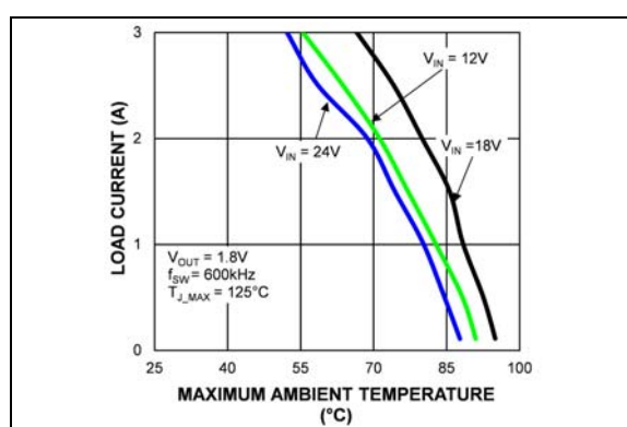
FIGURE 2-38: Thermal Derating (MIC28303-2).
