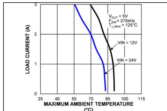
FIGURE 2-3: Thermal Derating (MIC28303-2).
