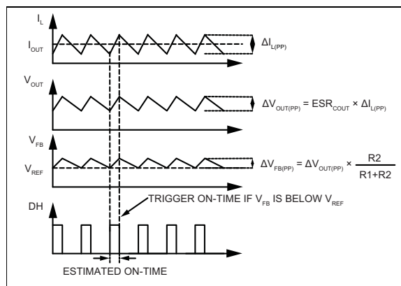
FIGURE 4-1: MIC28303 Control Loop Timing
