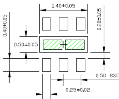
RECOMMENDED LAND PATTERN NOTE: 4
