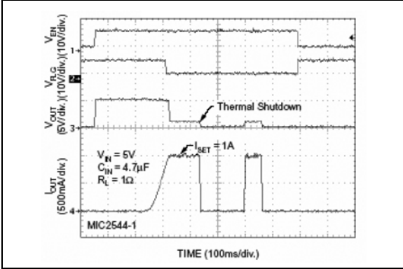
FIGURE 2-17: Current-Limit Response.
