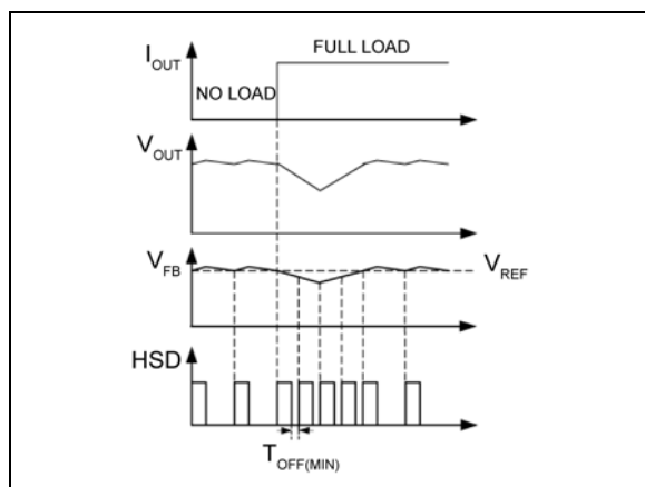
FIGURE 4-2: MIC24051 Load Transient Response.
