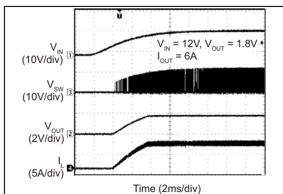
FIGURE 2-35: V_{IN} Soft Turn-On.
