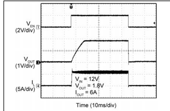
FIGURE 2-40: Enable Turn-On/Turn-Off.
