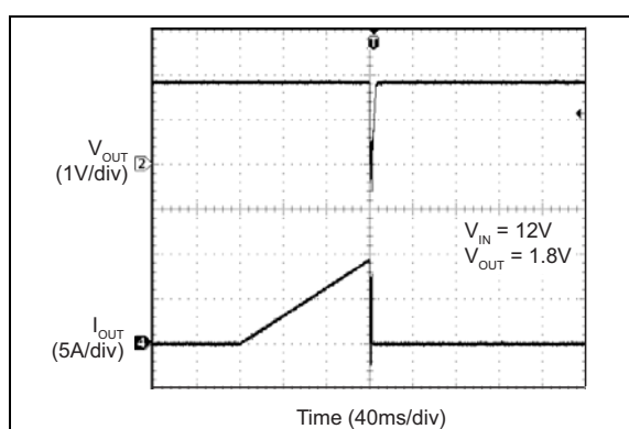
FIGURE 2-47: Output Current-Limit Threshold.
