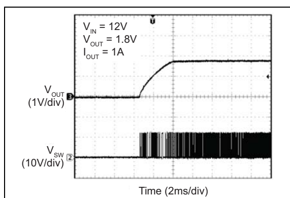
FIGURE 2-48: Output Recovery from Thermal Shutdown.
