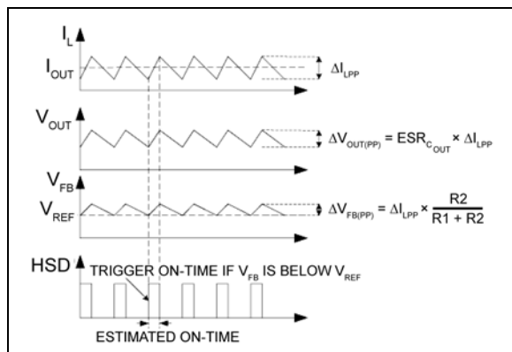
FIGURE 4-1: MIC24051 Control Loop Timing.
