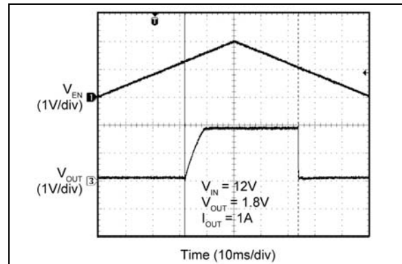
FIGURE 2-41: Enable Thresholds.
