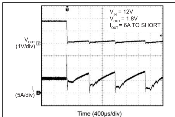
FIGURE 2-45: Short Circuit.
