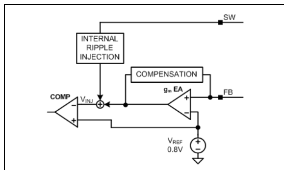
FIGURE 5-5: Internal Ripple Injection.
