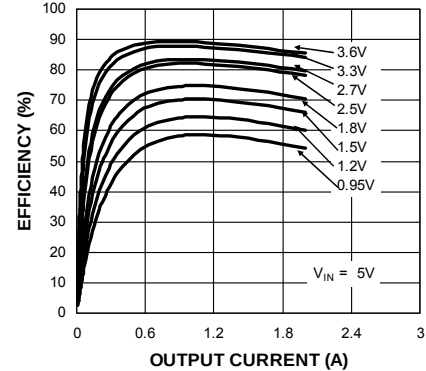
Efficiency ( V_{\text{IN}} = 5\text{V} ) vs. Output Current
