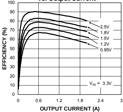
Efficiency ( V_{\text{IN}} = 3.3\text{V} ) vs. Output Current
