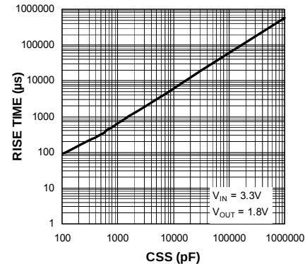
V_{\text{OUT}} Rise Time vs. C_{\text{SS}}
