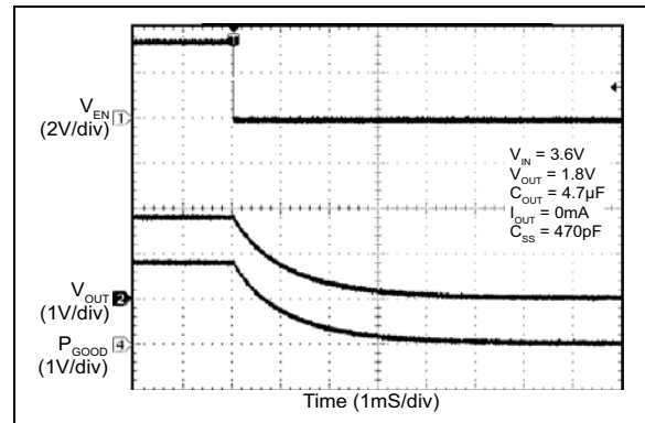
FIGURE 2-29: Power Good During Shutdown (MIC23159).
