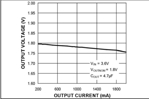
FIGURE 2-11: Load Regulation (CCM).
