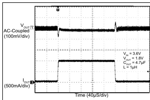
FIGURE 2-21: Load Transient (50 mA to 1A).
