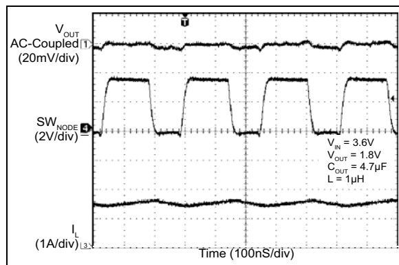
FIGURE 2-19: Switching Waveform Continuous Mode (1.5A).
