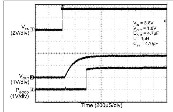
FIGURE 2-28: Power Good During Startup.
