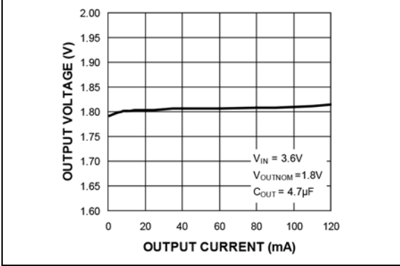
FIGURE 2-12: Load Regulation (HLL).
