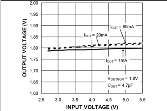
FIGURE 2-10: Line Regulation (HLL).
