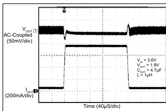
FIGURE 2-20: Load Transient (50 mA to 750 mA).
