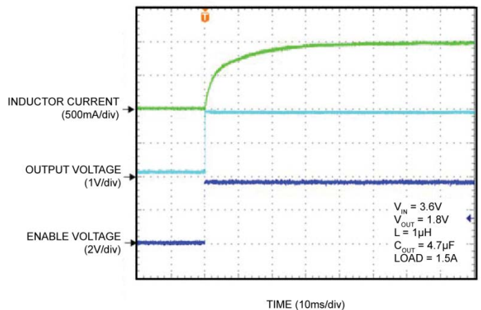
Start-Up Waveform
