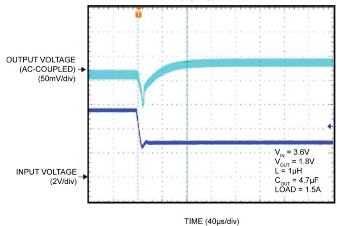
Line Transient 5.5V to 2.7V
