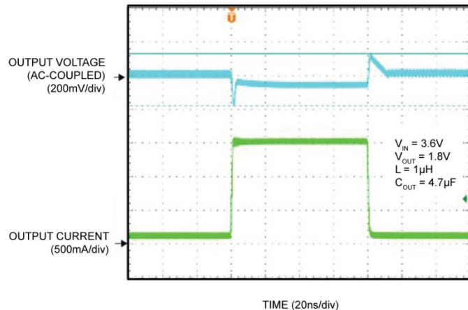
Load Transient 50mA to 1.5A
