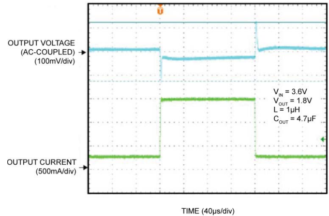
Load Transient 200mA to 1.5A
