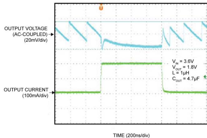
Load Transient 10mA to 200mA
