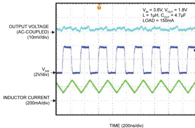
Switching Waveform Continuous Mode – 150mA
