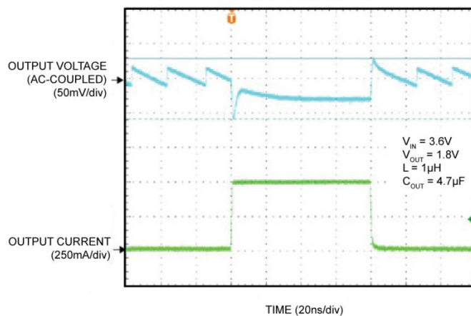
Load Transient 10mA to 500mA
