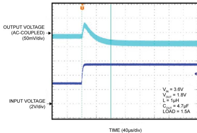
Line Transient 2.7V to 5.5V
