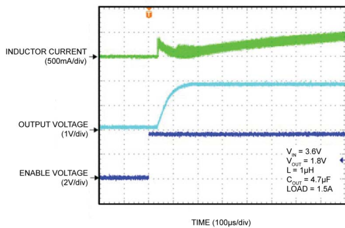
Turn-On Time
