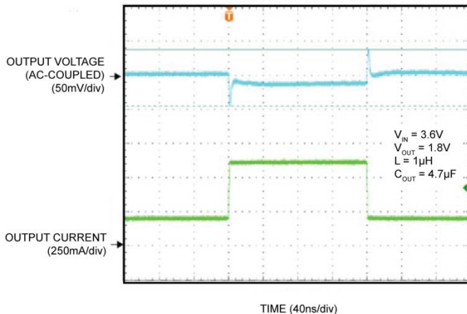
Load Transient 200mA to 600mA
