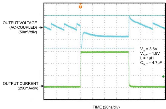
Load Transient 10mA to 750mA
