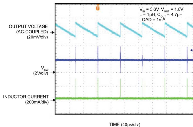
Switching Waveform Discontinuous Mode – 1mA
