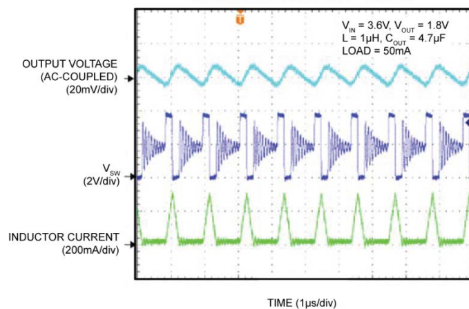
Switching Waveform Discontinuous Mode – 50mA
