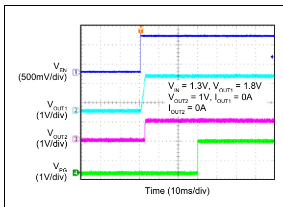
FIGURE 4-1: Power-up Sequencing.
