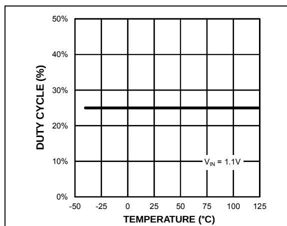
FIGURE 2-18: LED Flash Duty Cycle vs. Temperature.
