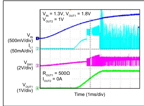
FIGURE 2-34: Power-up with 500Ω Load.
