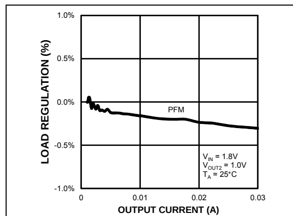
FIGURE 2-4: Buck Load Regulation vs. Output Current.
