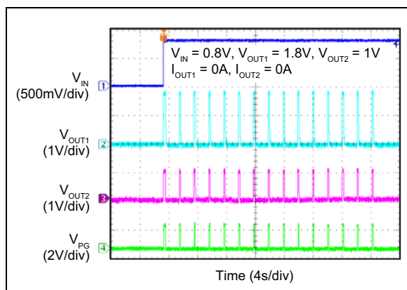
FIGURE 4-4: Low-Battery Power Cycling.
