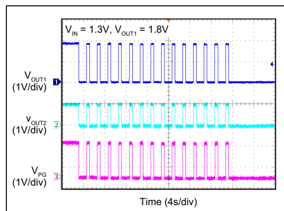
FIGURE 2-36: Short-Circuit Cycles – V_{OUT1} .
