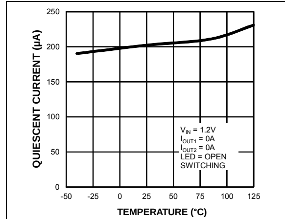
FIGURE 2-11: V_{IN} Quiescent Current (Switching) vs. Temperature.
