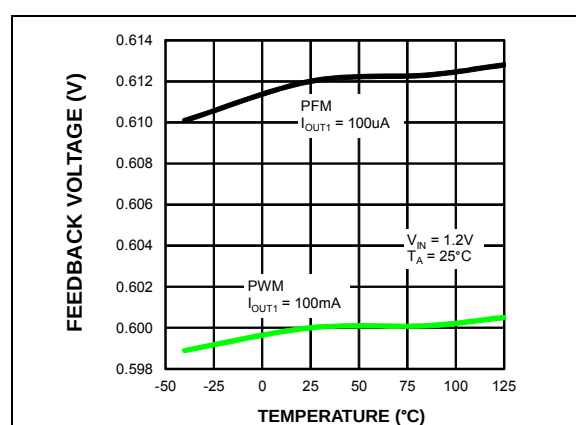
FIGURE 2-5: Boost Feedback Voltage vs. Temperature.
