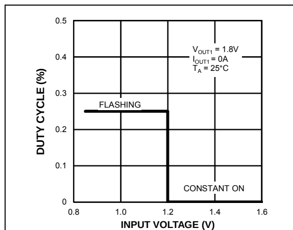
FIGURE 2-17: LED Flash Duty Cycle vs. Input Voltage.
