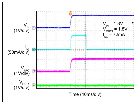
FIGURE 2-40: Power-up into Short Circuit – V_{OUT1} .
