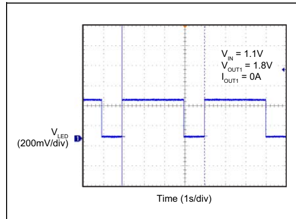
FIGURE 2-35: LED Flash Frequency and Duty Cycle.
