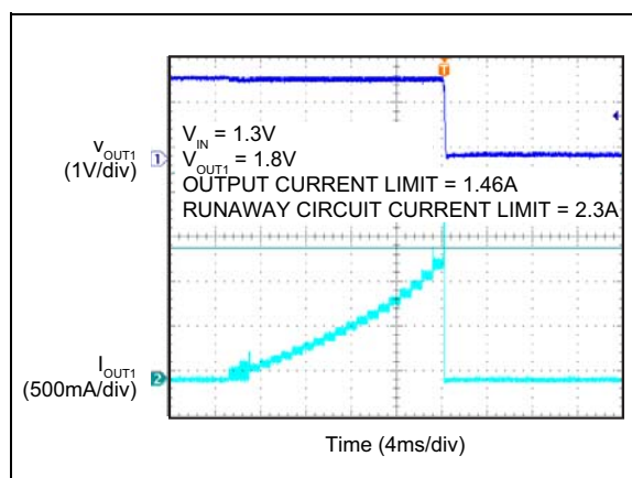
FIGURE 2-41: Boost Output Current Limit – V_{OUT1} .
