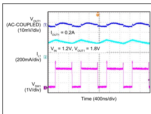
FIGURE 2-42: Boost Switching Waveforms – 200 mA.
