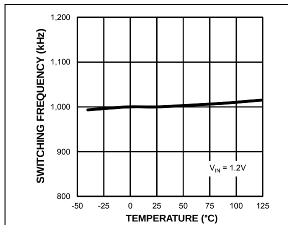
FIGURE 2-16: Boost Switching Frequency (PWM) vs. Temperature.
