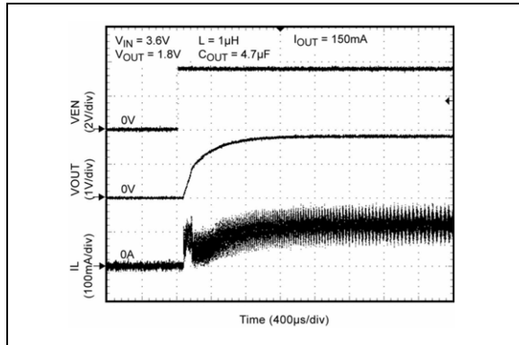
FIGURE 2-19: Start-Up Waveform.
