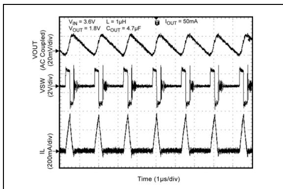
FIGURE 2-14: Switching Waveform.
