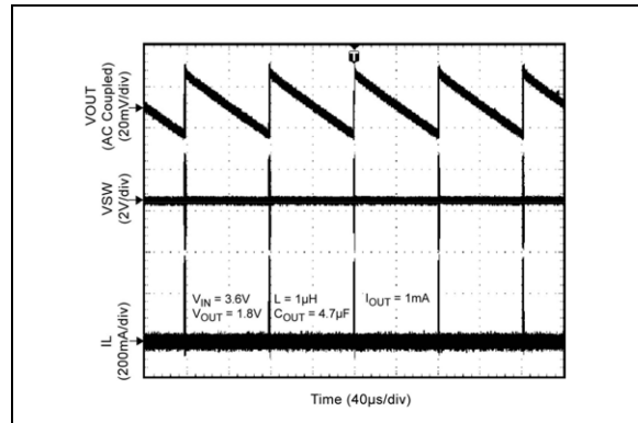
FIGURE 2-12: Switching Waveform.
