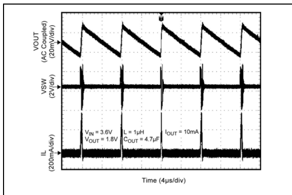
FIGURE 2-13: Switching Waveform.
