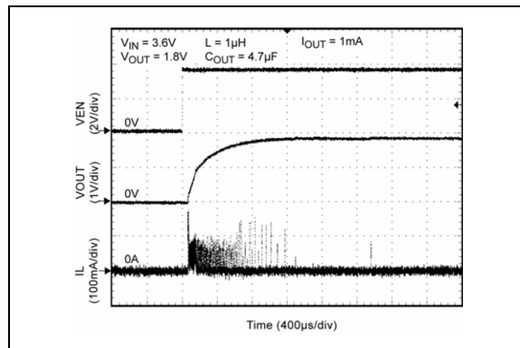
FIGURE 2-18: Start-Up Waveform.
