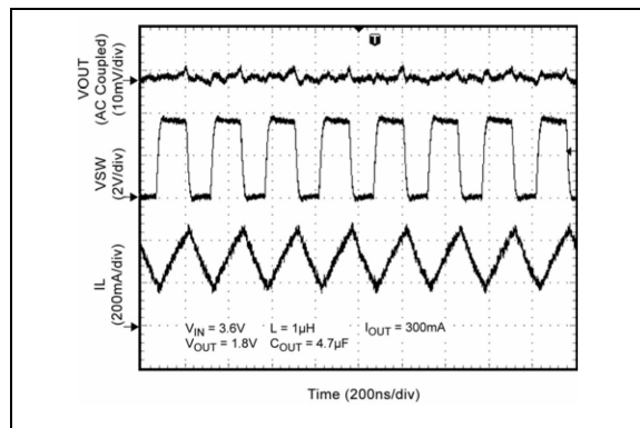
FIGURE 2-16: Switching Waveform.
