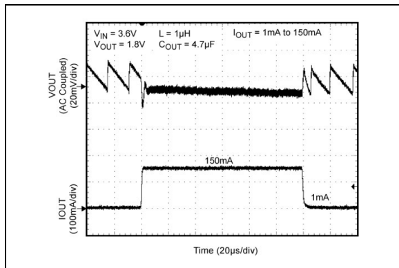
FIGURE 2-20: Load Transient.
