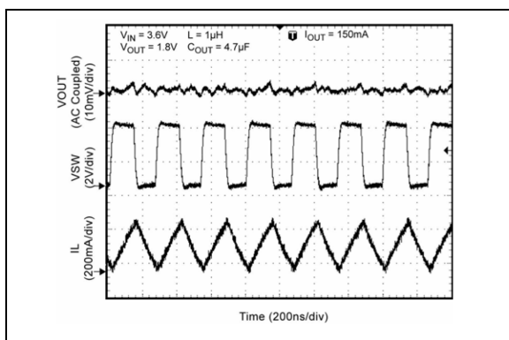
FIGURE 2-15: Switching Waveform.
