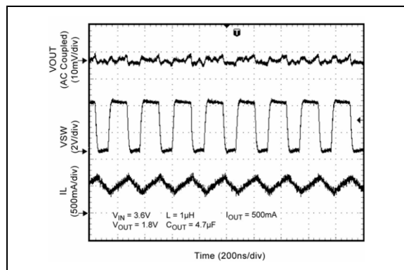
FIGURE 2-17: Switching Waveform.
