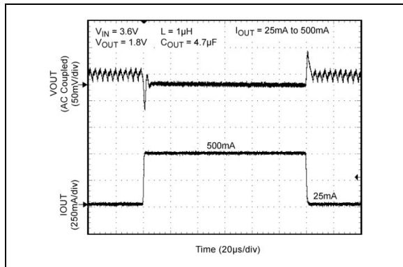
FIGURE 2-21: Load Transient.
