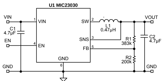
Figure 1. MIC23030-AYMT Schematic
