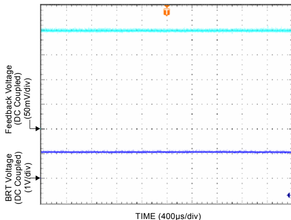
Figure 1. BRT = 1\text{V} , V_{FB} = 200\text{mV} , I_{LED} = 20\text{mA}
