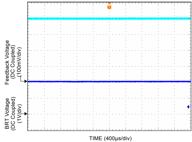
Figure 2. BRT = 2\text{V} , V_{FB} = 400\text{mV} , I_{LED} = 40\text{mA}
