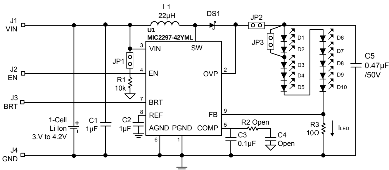
10 LED Configuration
