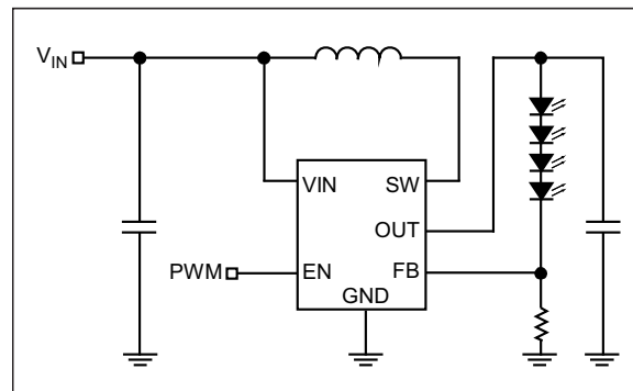
FIGURE 4-1: PWM Dimming Method.
