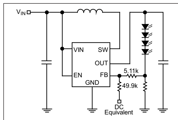
FIGURE 4-2: Continuous Dimming.
