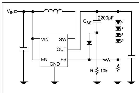
FIGURE 4-4: Soft-Start Circuit.
