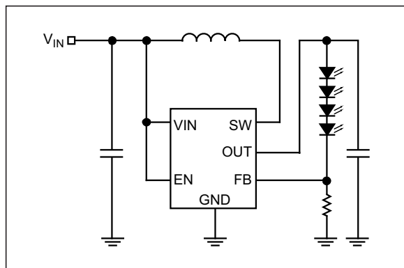
FIGURE 4-3: OVP Detection via OUT Pin.
