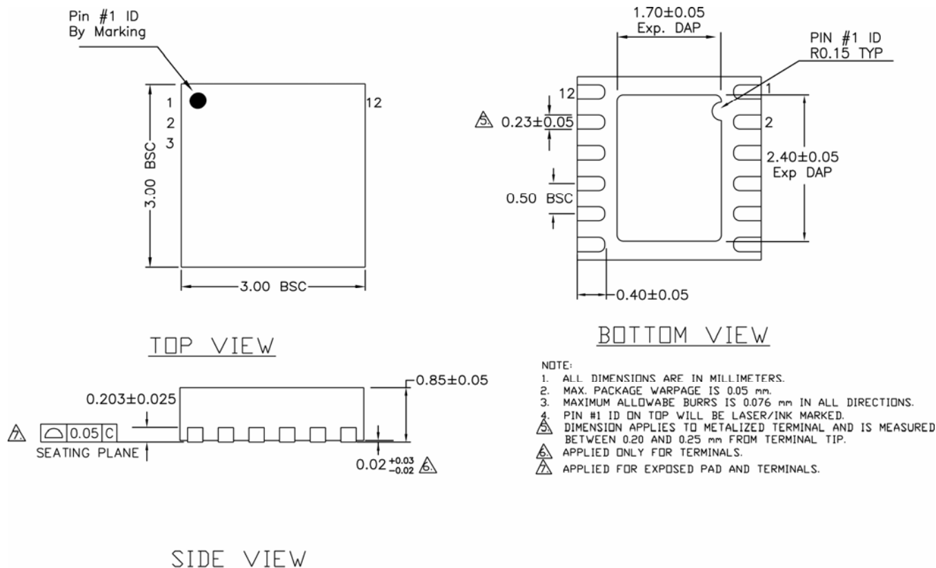
12-Pin 3mm × 3mm MLF® (ML)
