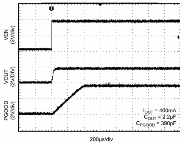
Enable Response
