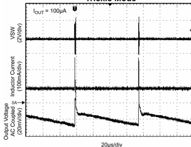
Switching Waveform Trickle Mode
