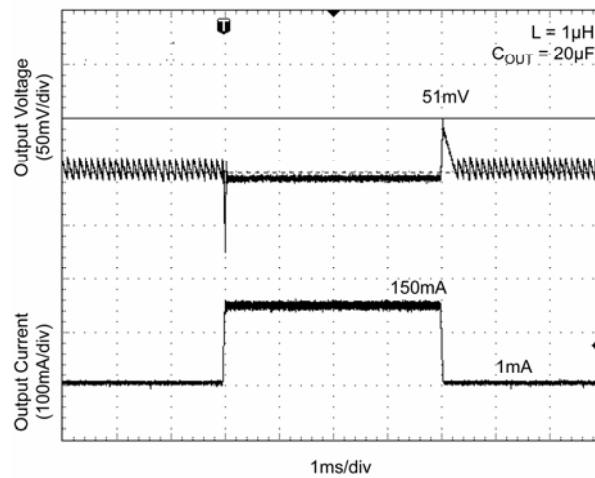
Transient Response
