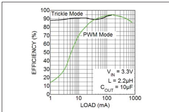
FIGURE 2-3: Efficiency.
