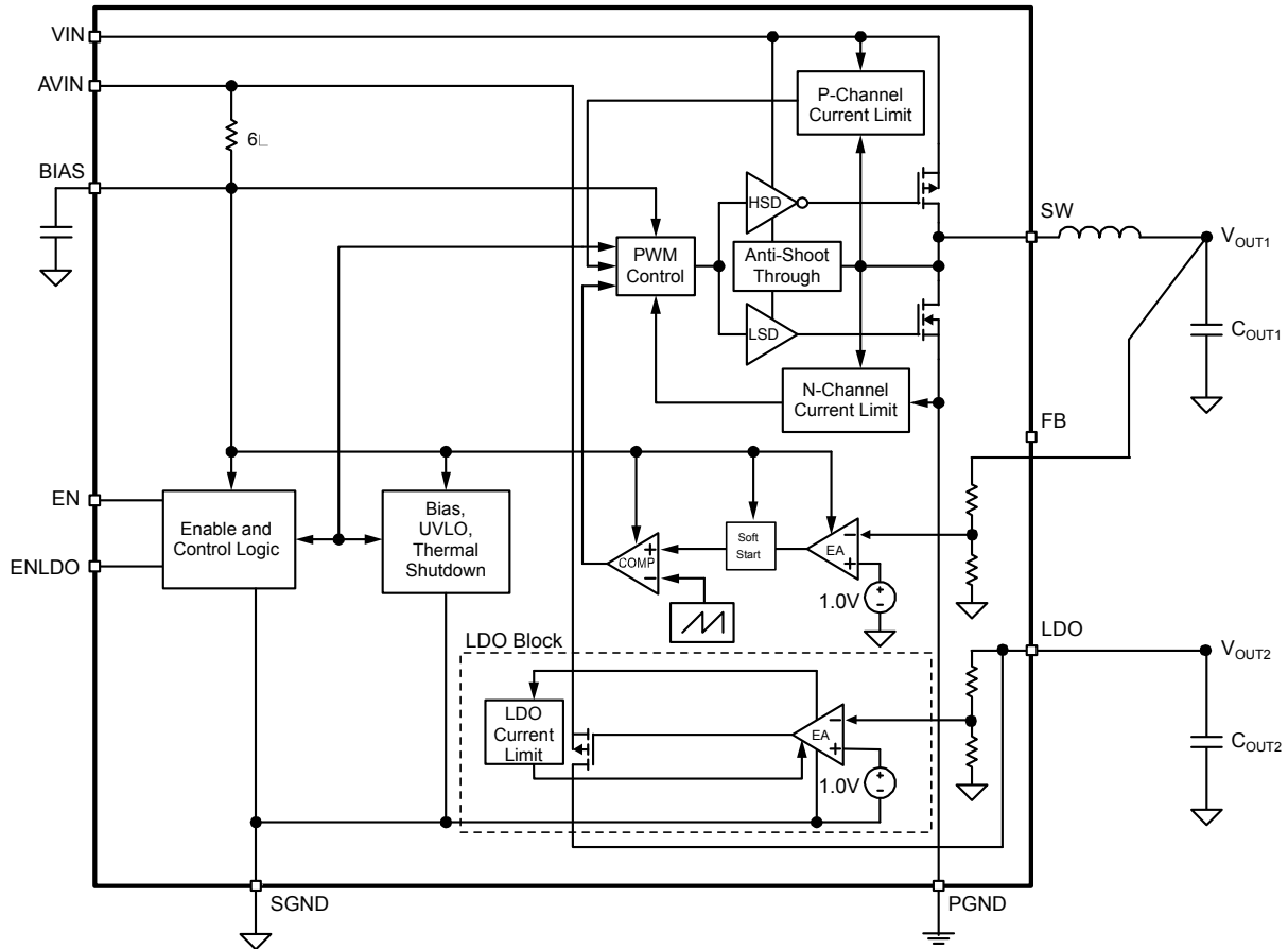
MIC2225 Block Diagram
