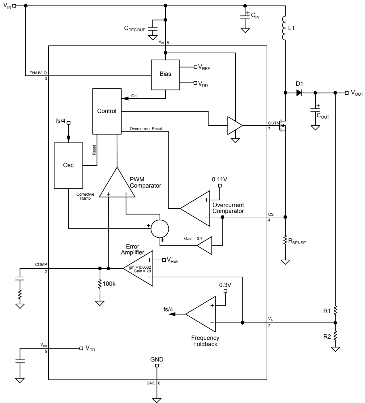
Figure 1. MIC2196 Block Diagram
