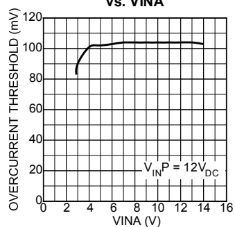
Overcurrent Threshold vs. V_{INA}
