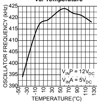
Oscillator Frequency vs. Temperature
