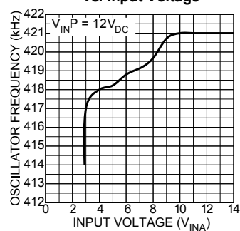
Oscillator Frequency vs. Input Voltage
