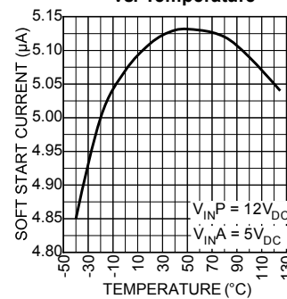
Soft Start Current vs. Temperature
