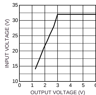
Figure 11. Max. Input Voltage in Forced-PWM Mode
