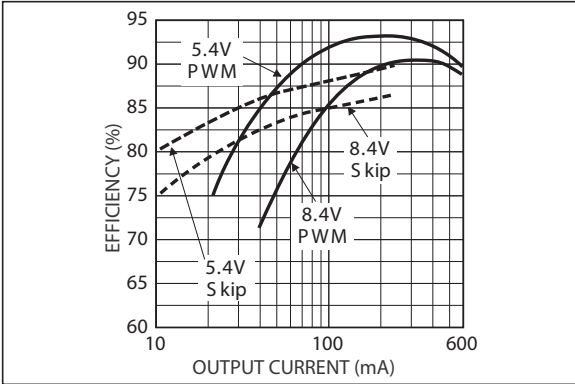
FIGURE 2-11: Skip-Mode and PWM-Mode Efficiency.
