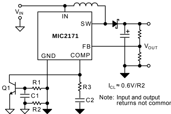
Figure 4. Current Limit
