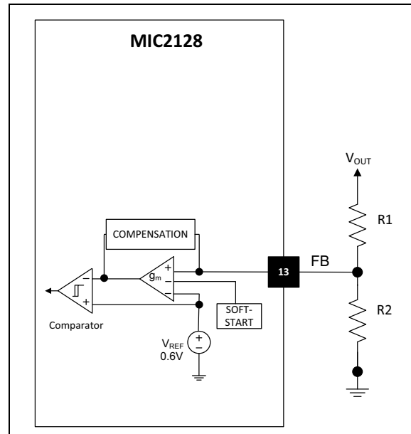
FIGURE 5-3: Output Voltage Adjustment.
