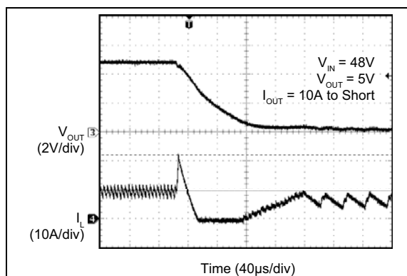
FIGURE 2-59: Short-Circuit.
