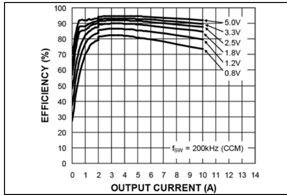
FIGURE 2-12: Efficiency ( V_{IN} = 18V ) vs. Output Current (MIC2103).
