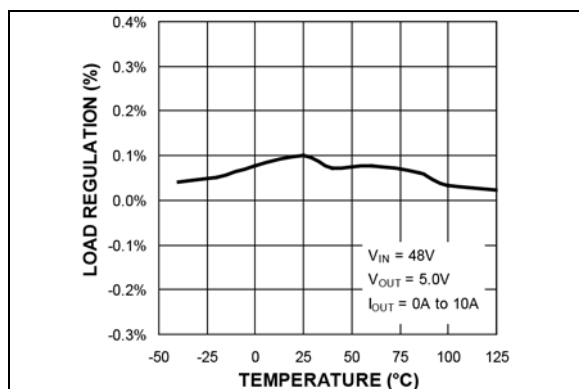
FIGURE 2-7: Load Regulation vs. Temperature (MIC2103).
