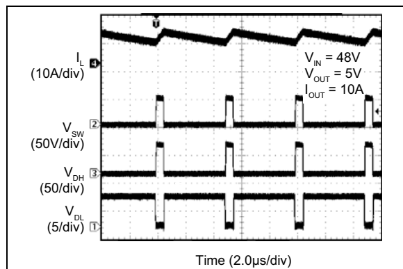
FIGURE 2-67: MIC2103 Switching Waveforms ( I_{OUT} = 10A ).
