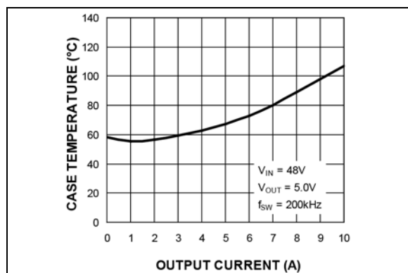
FIGURE 2-32: Case Temperature* ( V_{IN} = 48V ) vs. Output Current.
