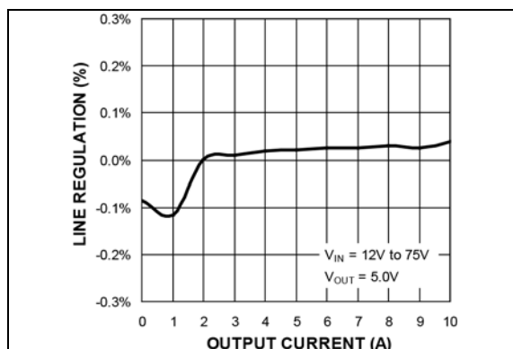
FIGURE 2-10: Line Regulation vs. Output Current (MIC2103).
