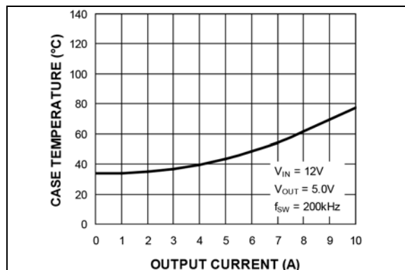
FIGURE 2-31: Case Temperature* ( V_{IN} = 12V ) vs. Output Current.
