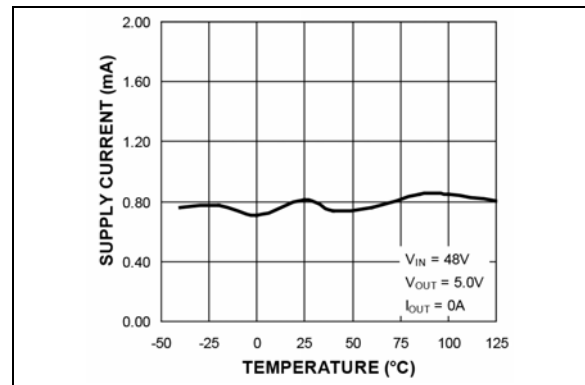
FIGURE 2-5: V_{IN} Operating Supply Current vs. Temperature (MIC2103).
