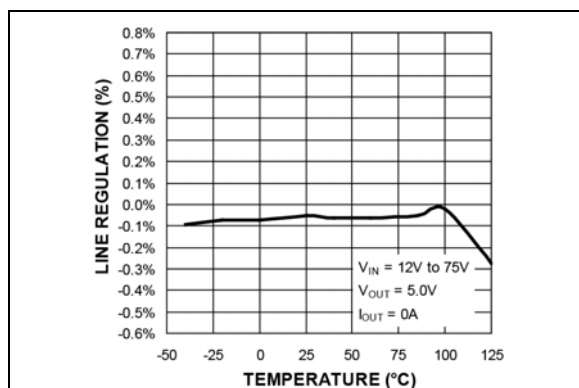
FIGURE 2-8: Line Regulation vs. Temperature (MIC2103).
