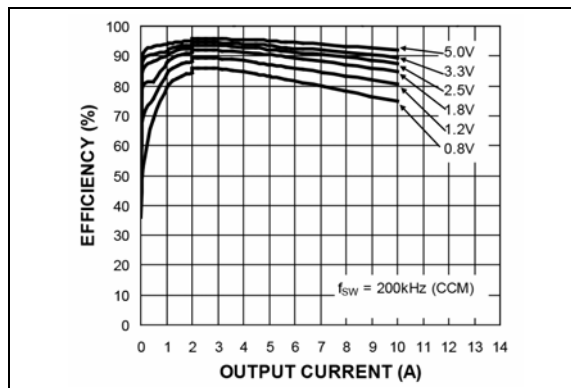
FIGURE 2-11: Efficiency ( V_{IN} = 12V ) vs. Output Current (MIC2103).
