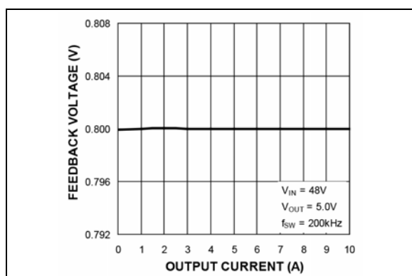
FIGURE 2-9: Feedback Voltage vs. Output Current (MIC2103).
