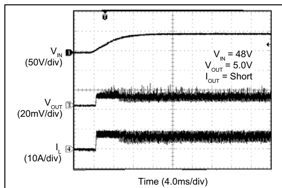
FIGURE 2-57: Power-Up into Short-Circuit.
