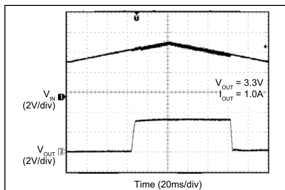
FIGURE 2-56: V_{IN} UVLO Thresholds.
