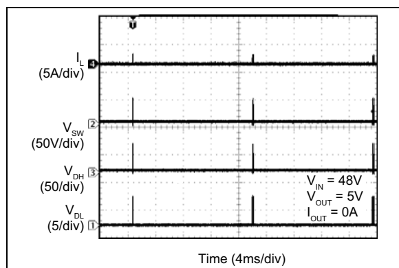
FIGURE 2-68: MIC2103 Switching Waveforms ( I_{OUT} = 0A , DCM).
