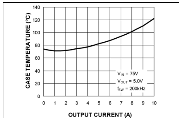
FIGURE 2-33: Case Temperature* ( V_{IN} = 75V ) vs. Output Current.
