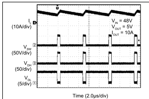
FIGURE 2-69: MIC2104 Switching Waveforms ( I_{OUT} = 10A ).
