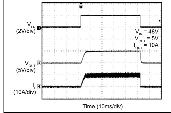
FIGURE 2-54: Enable Turn-On/Turn-Off.
