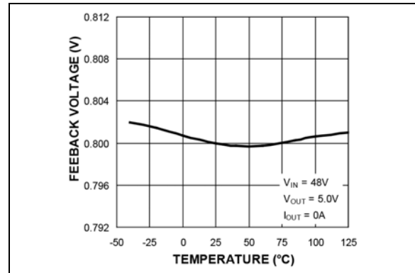
FIGURE 2-40: Feedback Voltage vs. Temperature.
