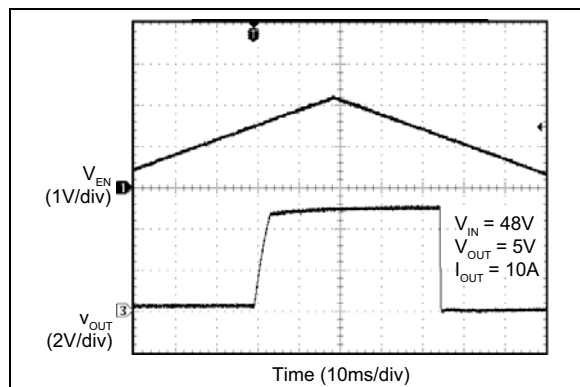
FIGURE 2-55: Enable Thresholds.
