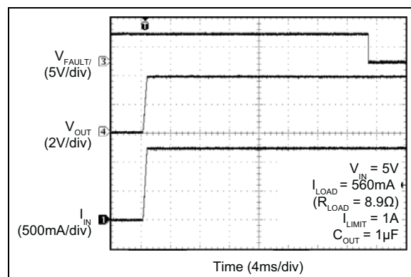
FIGURE 2-28: Turn-On into 12% Overload - 500 mA I_{LIMIT} .
