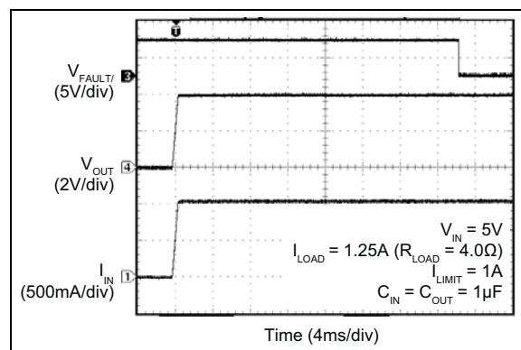
FIGURE 2-29: Turn-On into 25% Overload - 1A I_{LIMIT} .
