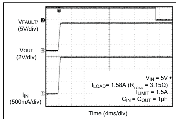
FIGURE 2-30: Turn-On into Minimal Overload - 1.5A I_{LIMIT} .
