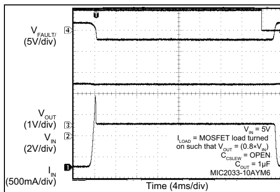
FIGURE 2-24: Current-Limit Response.
