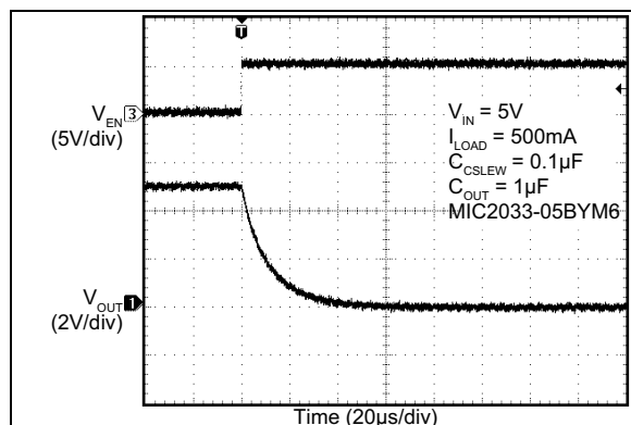
FIGURE 2-21: Enable Turn-Off.
