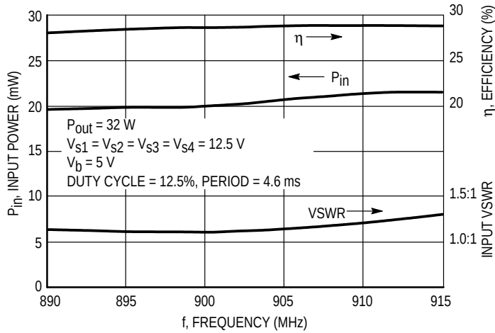
Figure 2. Input Power, Efficiency and Input VSWR versus Frequency
