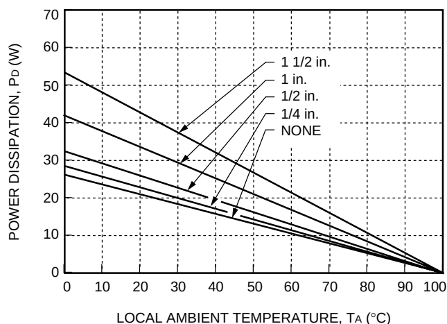
Figure 9. Heat Sink Power Derating Curves Natural Convection, Transverse Ori- entation
