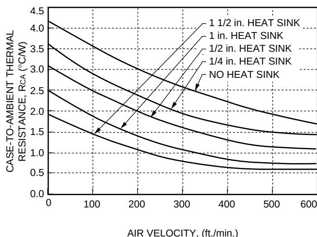
Figure 11. Case-to-Ambient Thermal Resistance Curves, Longitudinal Orientation
