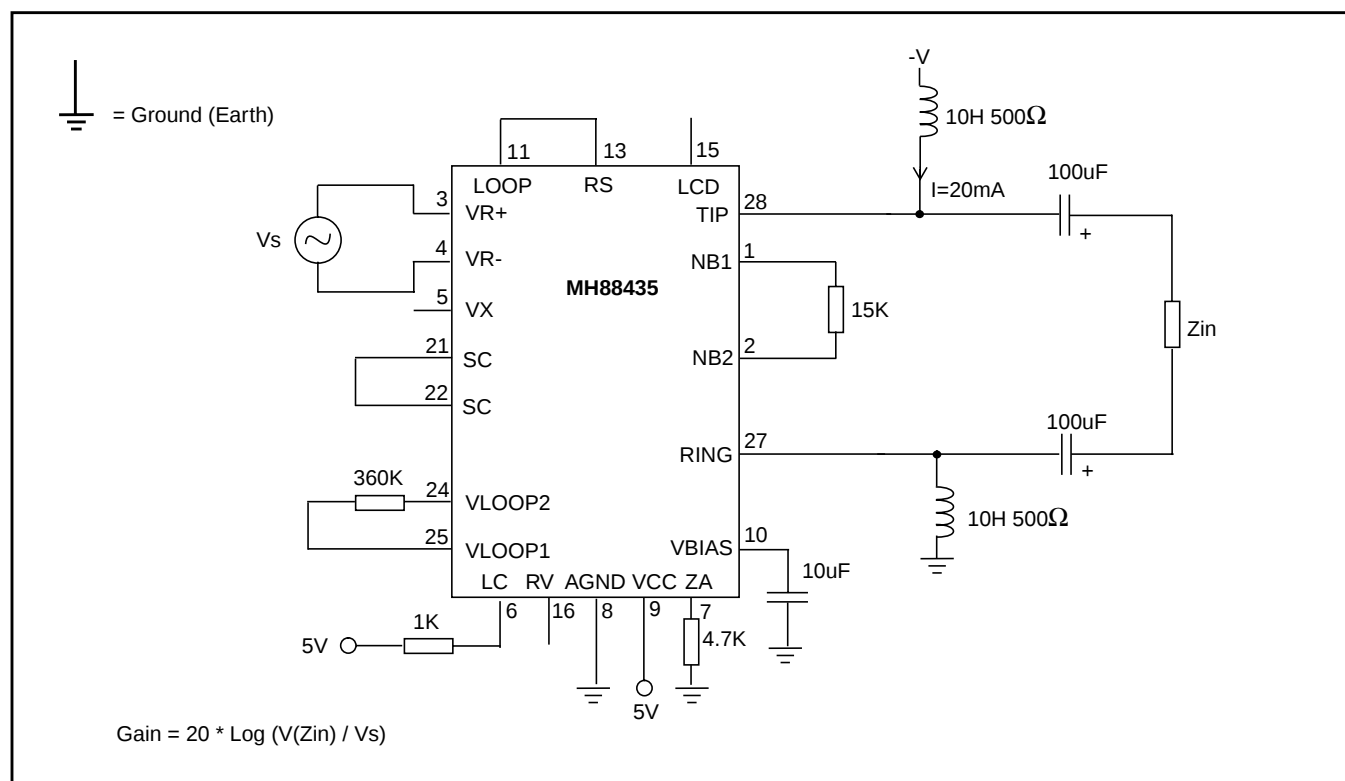
Figure 8 - Test Circuit 3
