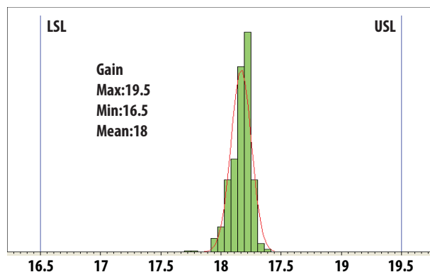
Figure 4. Gain @ 900MHz, 5V, 54mA Mean = 18
