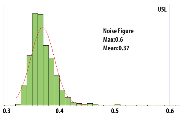
Figure 2. Noise Figure @ 900MHz, 5V, 54mA Mean = 0.37
