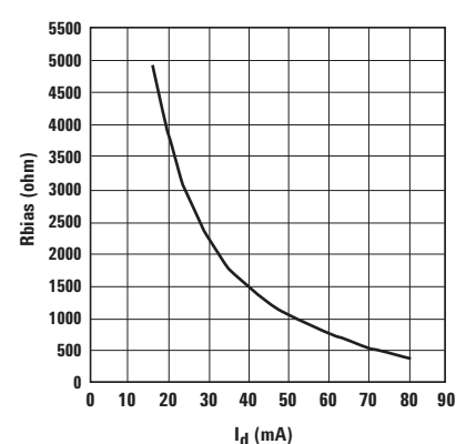
Figure 7. Rbias vs. I_d (5V supply).
