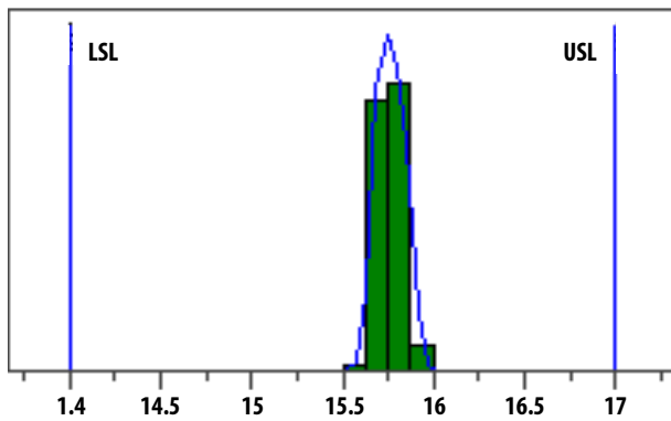
Figure 6. Gain Distribution
