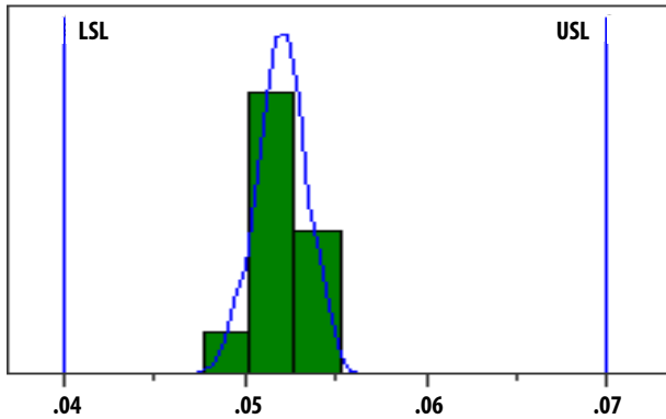
Figure 2. Idd Distribution
