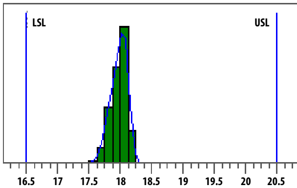
Figure 4. P1dB Distribution
