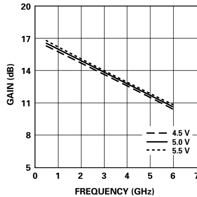
Figure 13. Gain vs. Frequency and Temperature.
