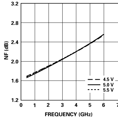
Figure 10. Noise Figure vs. Frequency and Voltage.
